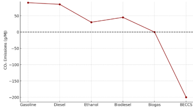
Fig. 4. Life-cycle greenhouse gas emissions of biomass pathways compared to fossil fuels.
