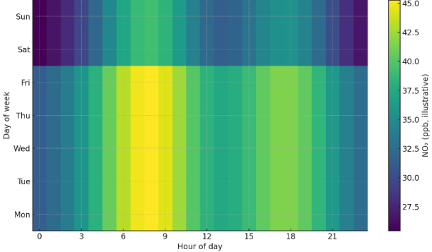
Fig. 2. diurnal-weekly NO_2 pattern (hour \times weekday)
