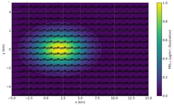
Fig. 4. synthetic urban plume with wind vectors
