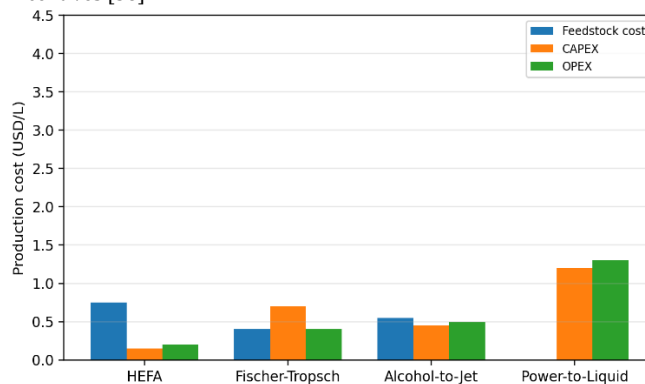
Fig 4. SAF Production Cost Breakdown by Pathway
