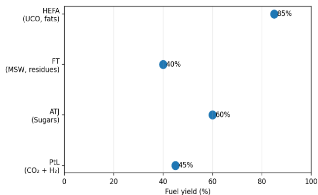
Fig 2. Fuel Yields by SAF Pathway.
