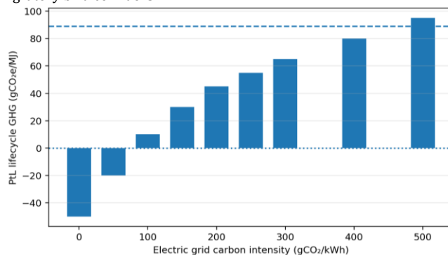
Fig 7. Sensitivity of PtL GHG Emissions to Grid Carbon Intensity
